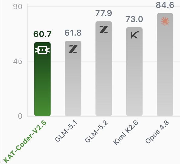
Terminal-Bench 2.1 AA Coding Index
