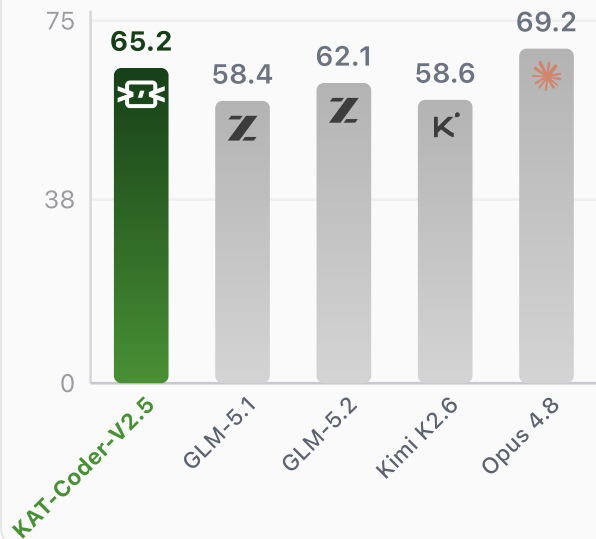
SWE-Bench Pro Coding
